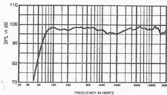
FIGURE 2 - DMC-1122B/DML-1122A Axial Frequency Response (1 watt/1 meter into LF midband)
