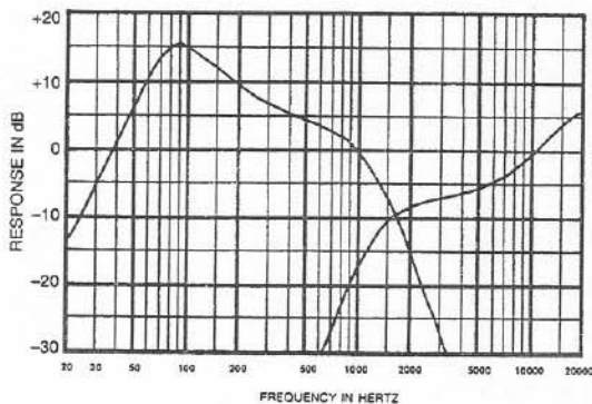
FIGURE 1 - DMC-1122B Frequency Response
