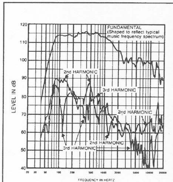
FIGURE 6 - DMC-1122B/DML-1122A Harmonic Distortion (115 dB SPL/1 meter using typical music frequency spectrum)
