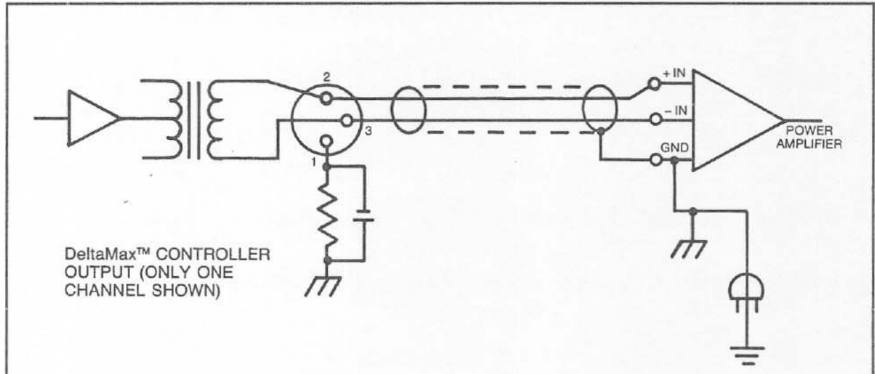
FIGURE 7 - DeltaMax™ Output Connection
